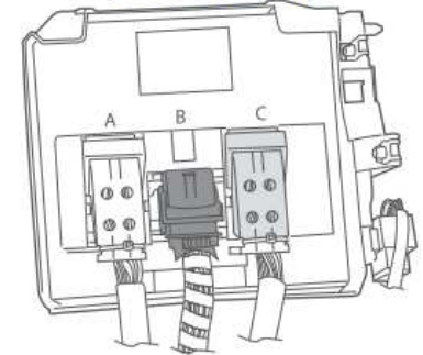
Body Control Module
